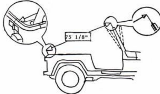
Figure 2 – Windshield distance
